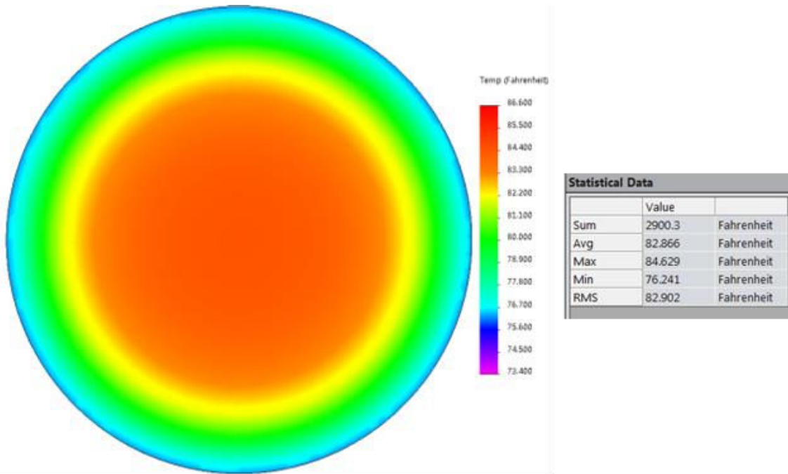
Figure 7: Uniform Heater Simulation Results after 10 minutes and 5 volts Input Voltage
