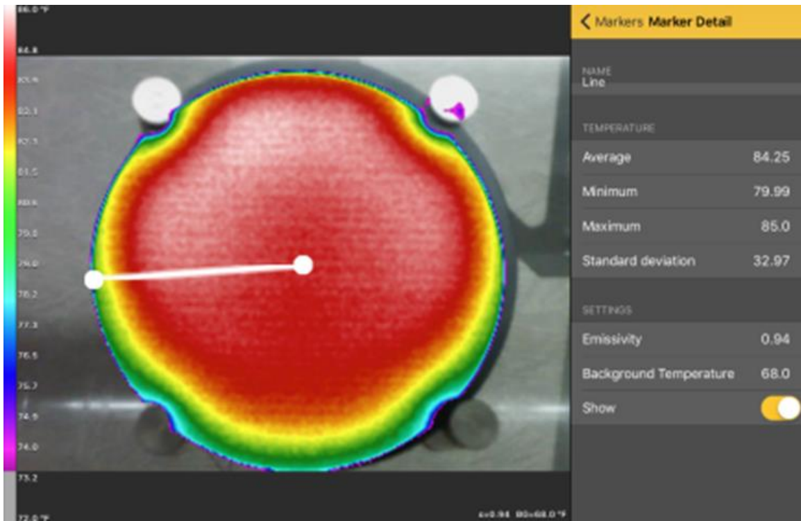
Figure 6: Thermal image of a profiled heater after 10 minutes and 5 volts input voltage
