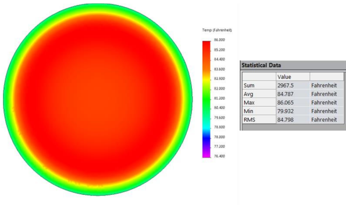
Figure 5: Profiled heater simulation results after 10 minutes and 5 volts input voltage
