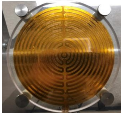
Figure 3: Heater Mounted with Standoffs to Back Face of Disc
