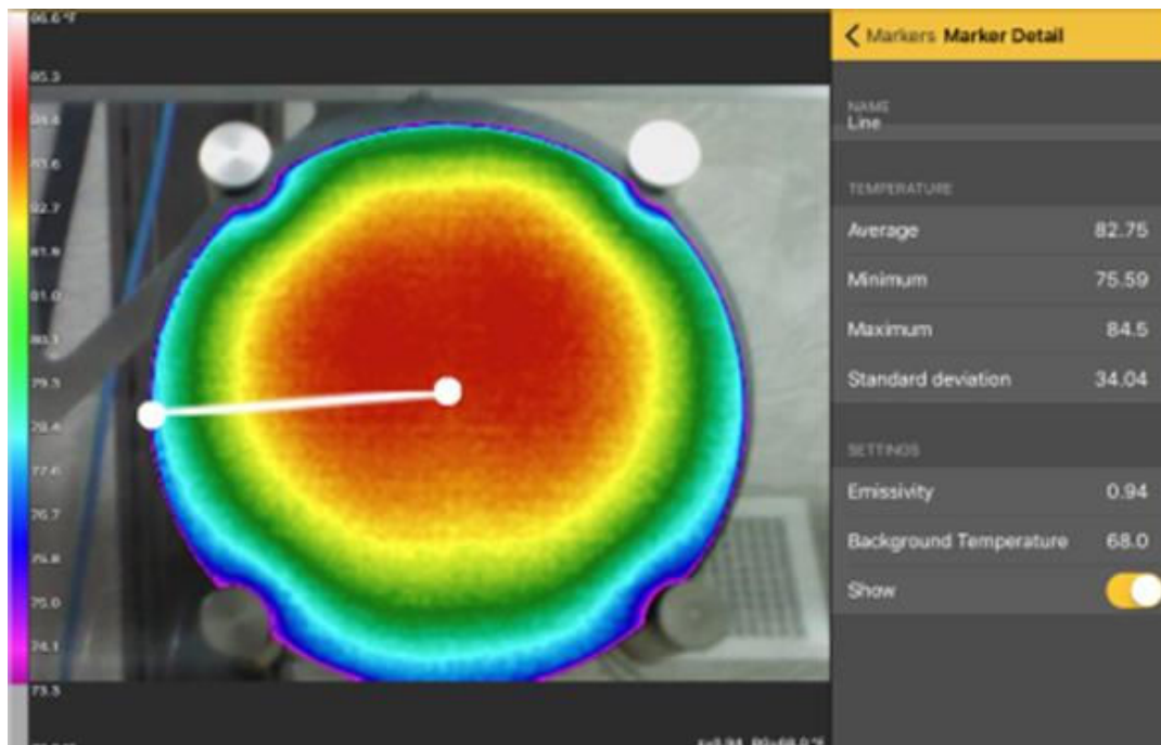
Figure 8: Thermal Image of Uniform Heater After 10 Minutes and 5 Volts Input Voltage
