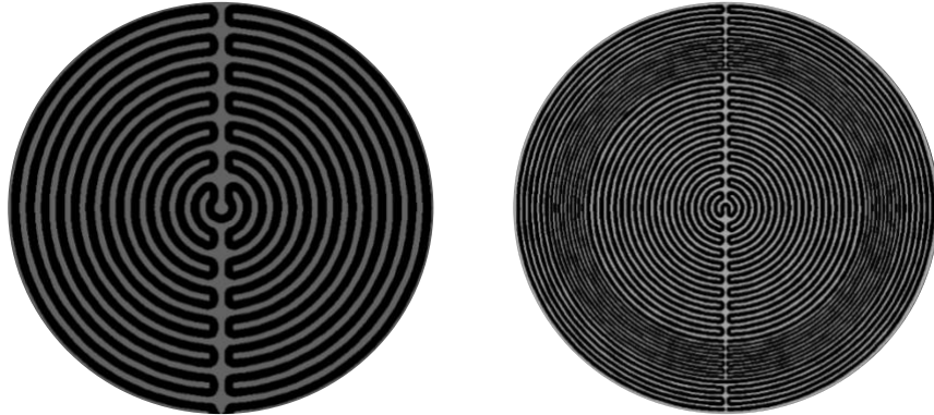
Figure 1: Uniform Heater Trace Layout (Left), Profiled Heater Trace Layout (Right)
