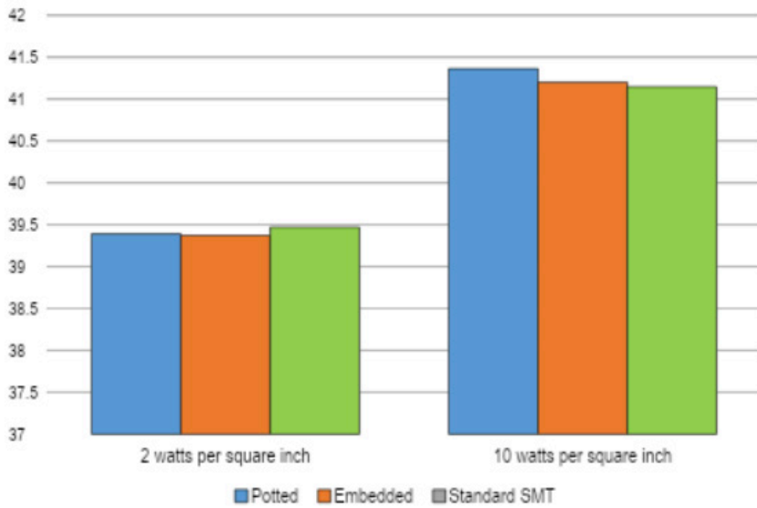
Maximum Overshoot with Control Temp at 37C
